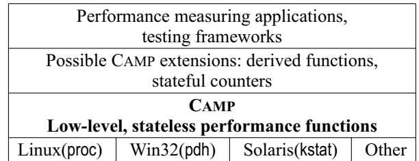
Figure 2: The CAMP system architecture.
