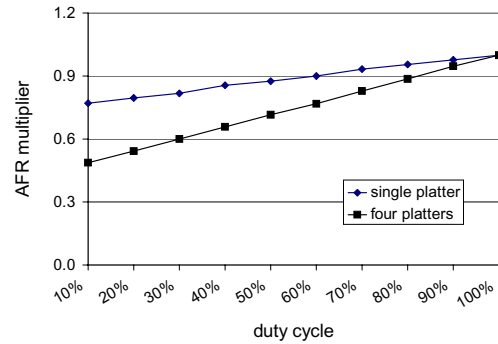
Figure 10: Reliability is decreased with higher duty cycle, and the effect is greater for drives with larger numbers of platters [Cole00].
