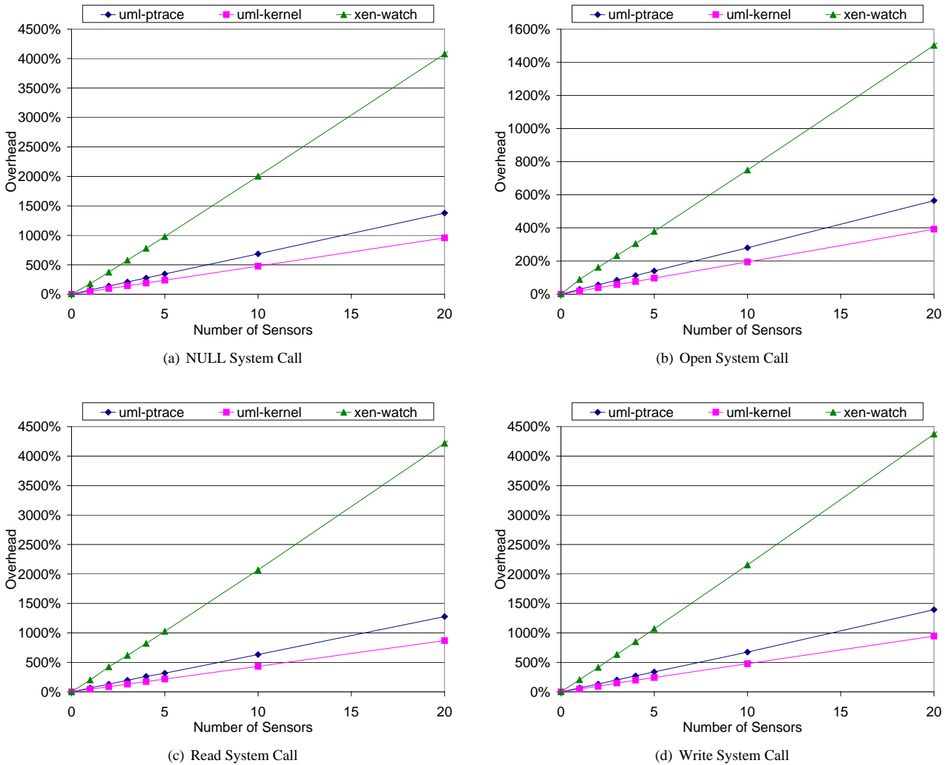
Figure 4. Scaling results for four LMBench microbenchmarks. These graphs plot the overhead the microbenchmarks experience as the number of sensors along the benchmark path was increased. Because Xen normally experiences better performance, the sensor mechanism introduces a greater amount of overhead.
