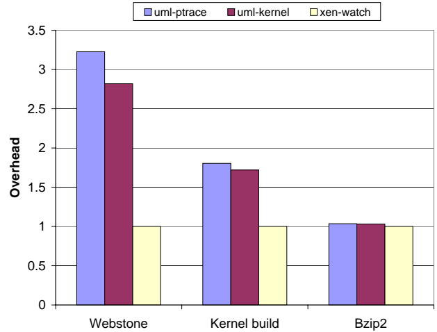
Figure 7. Execution times of implementations with sensors in Section 3 enabled. All execution times are normalized to the execution time in xen-watch .
