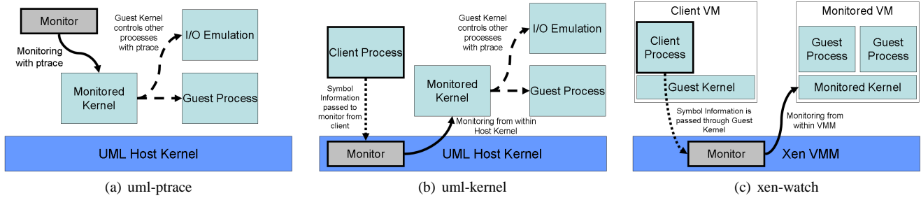
Figure 3. Architectural diagrams of uml-pttrace , uml-kernel and xen-watch illustrating the placement of the monitor and client process in relation to the monitored guest kernel and underlying VMM.
