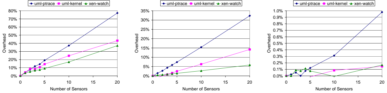
(a) Webstone Benchmark. There were 6.5K invocations/second in this benchmark. (b) Kernel Build Benchmark. There were 1.4K invocations/second in this benchmark. (c) Bzip2 Benchmark. There were 14 invocations/second in this benchmark.
