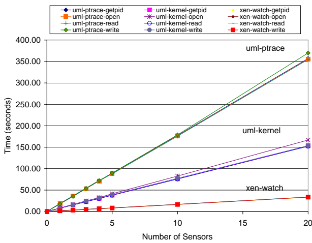
Figure 5. Incremental cost of monitoring as compared to the number of sensors placed along each benchmark execution path in the kernel.
