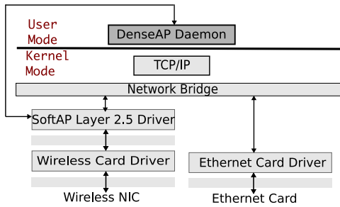
Figure 5. The network stack on each DenseAP node
