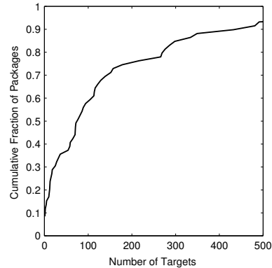
Figure 2: Cumulative distribution of the number of targets (servers) on which a software package is installed in several data centers. A larger number of packages are installed on only a small number of targets.
