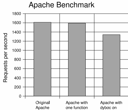
Figure 7: Apache benchmark results.
