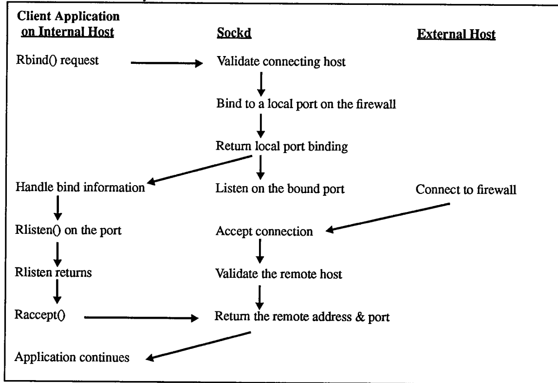
FIGURE 4. BIND Request
