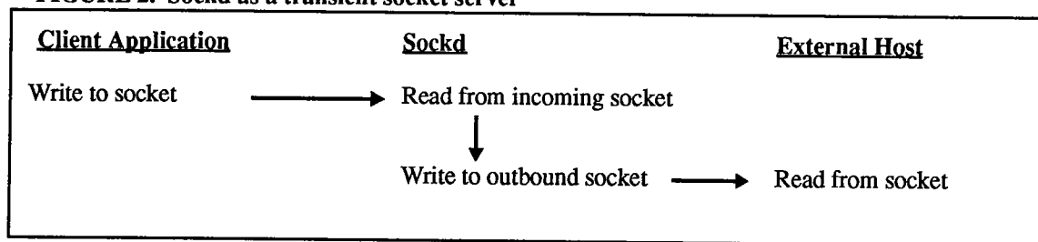
FIGURE 2. Sockd as a transient socket server
