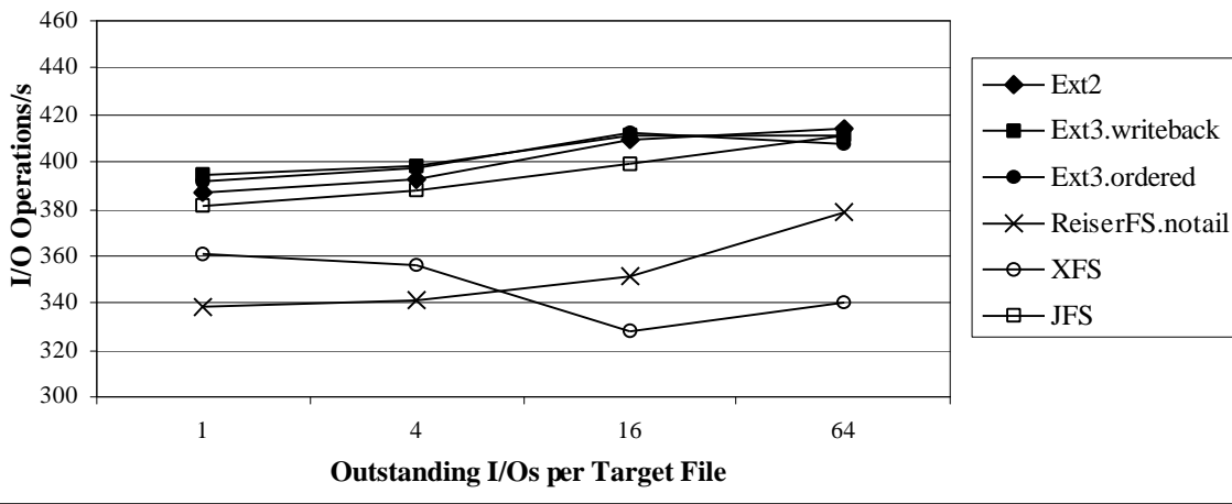
Figure 4: Pgmeter, Medium System, FileServer Workload
