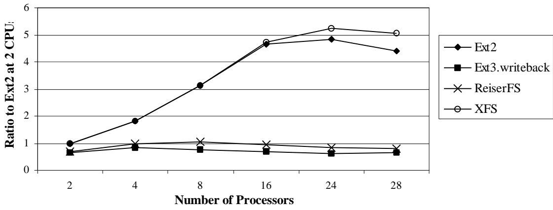
Figure 11: AIM7, Large System, 28-File Case
