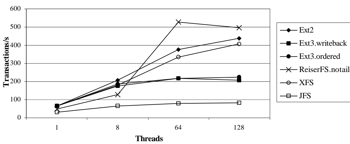
Figure 6: Filemark, Medium System, Small-File Workload
