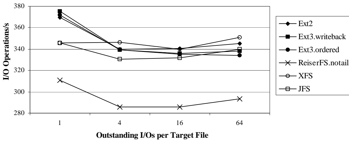
Figure 5: Pgmeter, Medium System, 8K OLTP Workload
