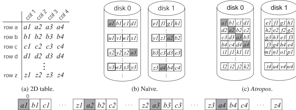
Figure 2: Two layouts for parallel access to a two-dimensional data structure mapped to a linear LBN address space.
