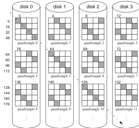
Figure 3: Atropos quadrangle layout. The numbers to the left of disk 0 are the VLBN s mapped to the gray disk locations connected by the arrow (not the first block of each quadrangle row). The arrow illustrates efficient access in the other-major.
