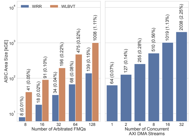
Figure 8: WLBVT and WRR exhibit linear area scaling in the GF 22nm process. Bar captions indicate gate count and relative area compared to 4 PU clusters with 4 MiB L2.
