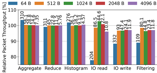
Figure 11: The relative packet throughput of common data-center workloads run in a standalone mode as a function of packet size with their raw performance in million packets per second (Mpps) at the top of the bars. Up to a 3% throughput increase with OSMOSIS compared to the PsPIN baseline stems from a kernel completion time variability introduced by the compute/IO schedulers.
