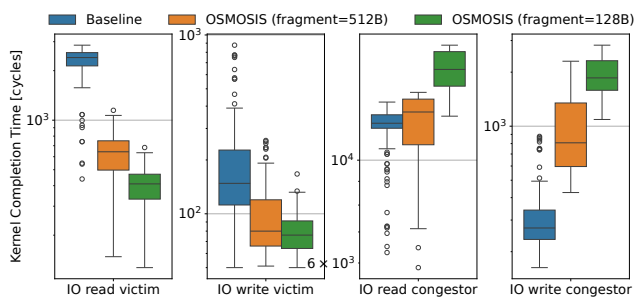
Figure 13: The completion time distribution for IO-bound applications for two fragment sizes.
