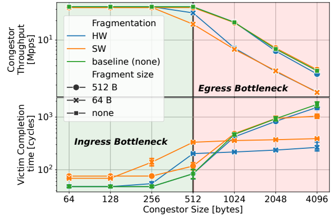
Figure 10: The impact on the Congestor throughput and the Victim kernel completion time as a function of the Congestor size and various fragment sizes. State transition between ingress and egress bottleneck depicts where the line rate of the egress path became saturated.
