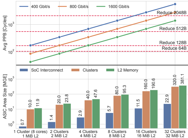
Figure 7: The cost model of sNIC SoC area synthesized in 22nm GF process, compared to the theoretical per packet budget (averaged for different packet sizes at 64 – 4096 B interval) achieved with 400/800/1600 Gbit/s ingress link rates.
