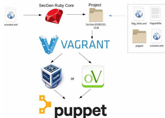
Figure 1: SecGen creates a project, then Vagrant creates VMs using VirtualBox or oVirt, and provisions via Puppet
