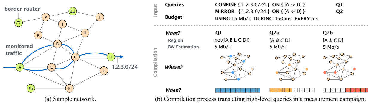
Figure 2: From high-level monitoring queries and the current network state, Stroboscope computes a measurement campaign schedule meeting the monitoring budget.
