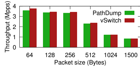
(b) Throughput in million-packets per second
