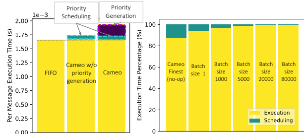
Figure 12: Cameo Scheduling Overhead.
