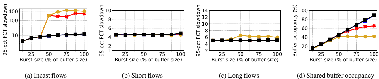
Figure 7: Performance of CREDENCE across various burst sizes of incast workload and websearch workload at 40% load, with DCTCP as the transport protocol. At small burst sizes, DT and ABM achieve similar performance compared to CREDENCE but as the burst size increases, CREDENCE outperforms DT and ABM in terms of FCTs for incast flows (burst absorption).
