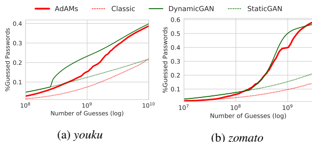
Figure A.2: Performance comparison between AdaMs and the dynamic attack [32]. Classic mangling rules attacks and StaticGAN [32] are reported as baseline.
