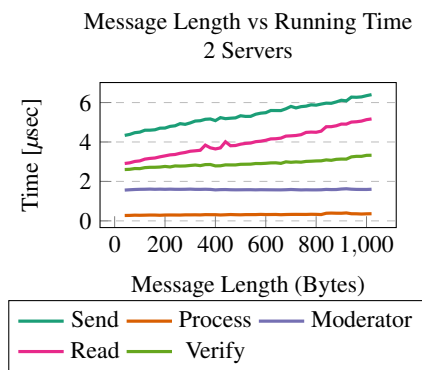
Figure 3: Running time as message length increases. Server-side operations on the critical path for message delivery run the fastest and do not noticeably increase in cost as message lengths increase.
