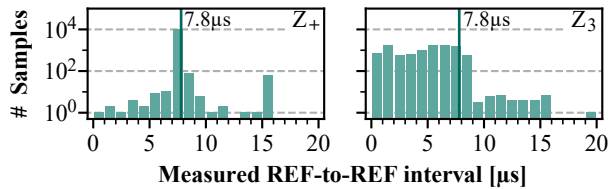
Figure 4. Measured time between successive REFs using the refresh synchronization routine ref_sync_original() , for both Z_+ and Z_3 . The number of samples (y-axis) are logarithmically scaled.
