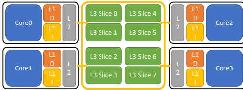
Figure 1: Diagram of Intel i7-7700 processor's cache and core structure. Each core has its own L1 and L2 caches. The L3 cache is shared between cores, and is split into slices.
