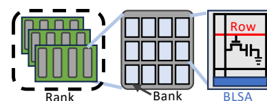
Figure 3: Diagram of DRAM organization
