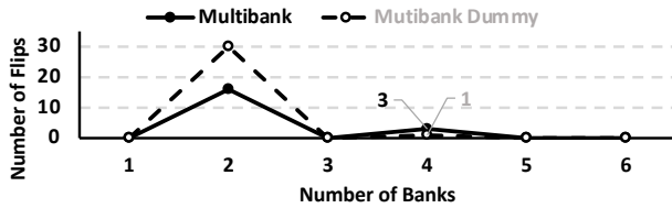
Figure 15: The total number of generated flips with Multibank and Multibank Dummy hammering on a 17-12700K CPU.
