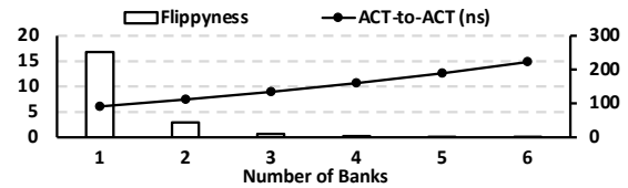
Figure 7: Results from Figure 6 divided by the number of banks and hammering iterations (flippyness) and the average time between two ACTs per bank (ACT-to-ACT).
