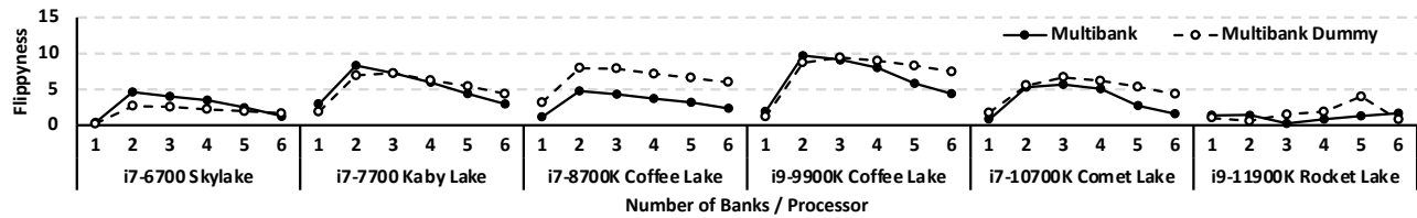
Figure 13: Flippiness of Multibank Hammering and Multibank Dummy Hammering across Processor generations.
