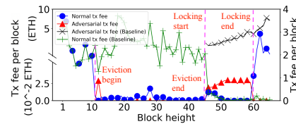
Figure 5: Evaluation of locking attack XT_8 on Reth
