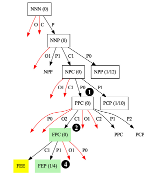
Figure 6: Snapshot of the MPFUZZ state-search tree when finding Exploit XT_6 on Geth v1.11.4.
