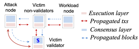
Figure 4: Experimental setup for locking attacks on Reth
